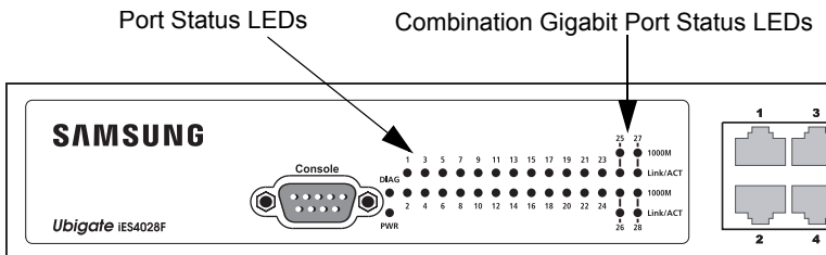
Figure 1-2 Port LEDs
