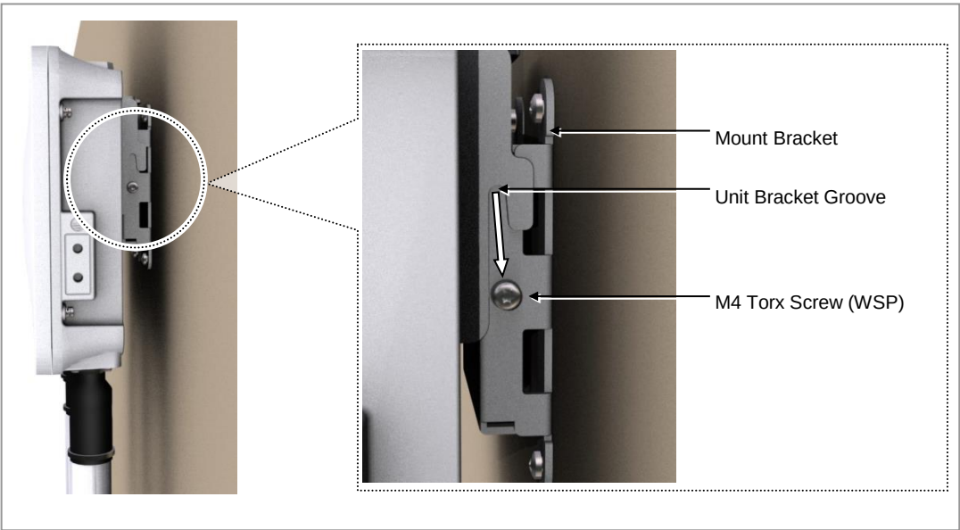
Figure 16. Mounting the Outdoor AP on the Wall (1)
