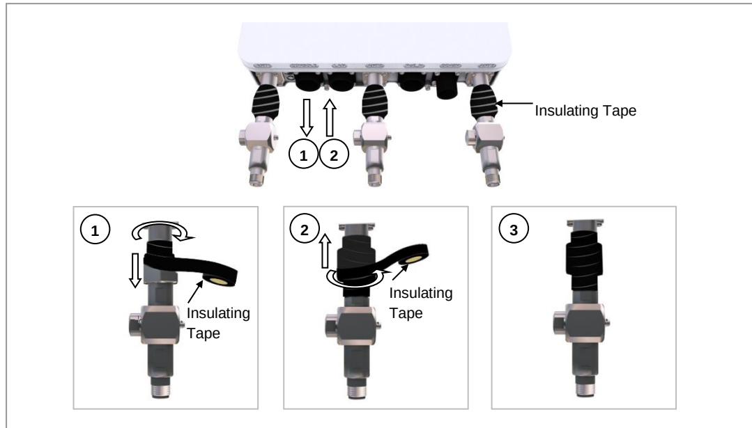
Figure 54. Connecting the Arrestors (2)
