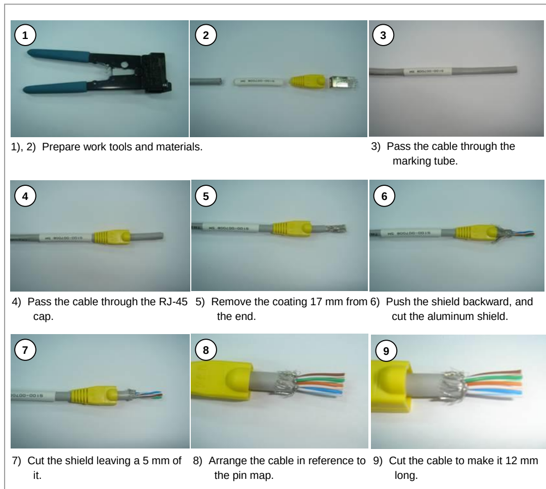
Figure 66. Assembling the RJ-45 Connector (Shield Type) (1)
