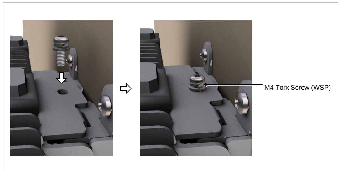
Figure 18. Mounting the Outdoor AP on the Wall (3)
