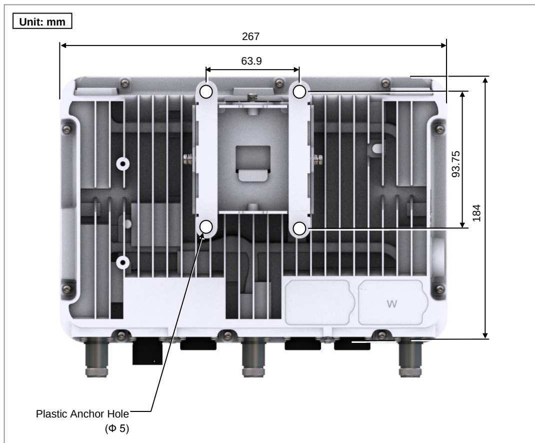
Figure 10. Marking the Outdoor AP
