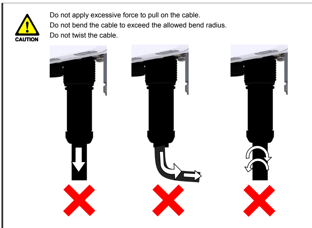
Figure 44. Connecting a Power Cable (3)
