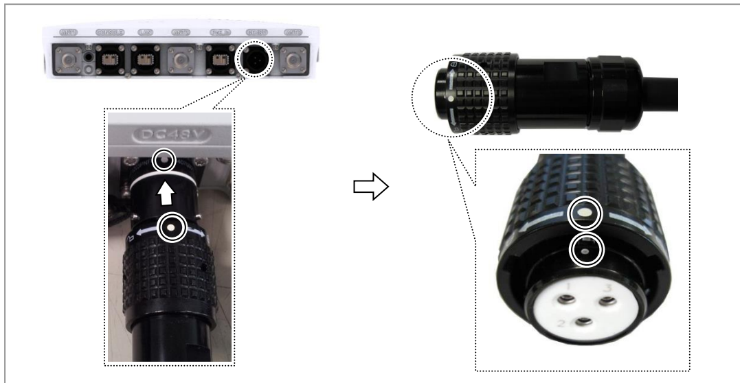
Figure 43. Connecting a Power Cable (2)
