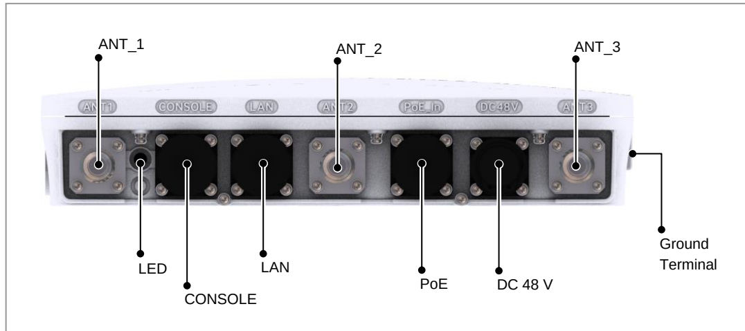
Figure 2. Outdoor AP Interface
