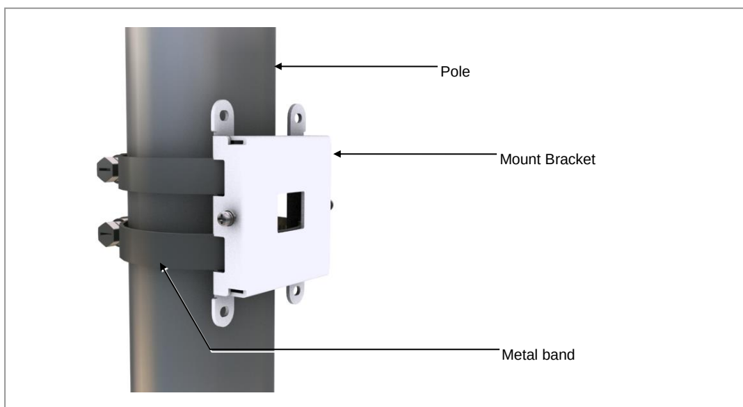
Figure 21. Mounting the Outdoor AP on a Pole (1)
