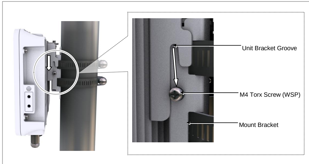
Figure 22. Mounting the Outdoor AP on a Pole (2)
