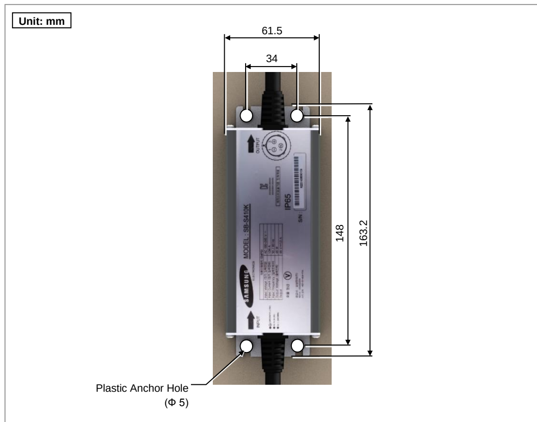
Figure 11. Marking the Adapter
