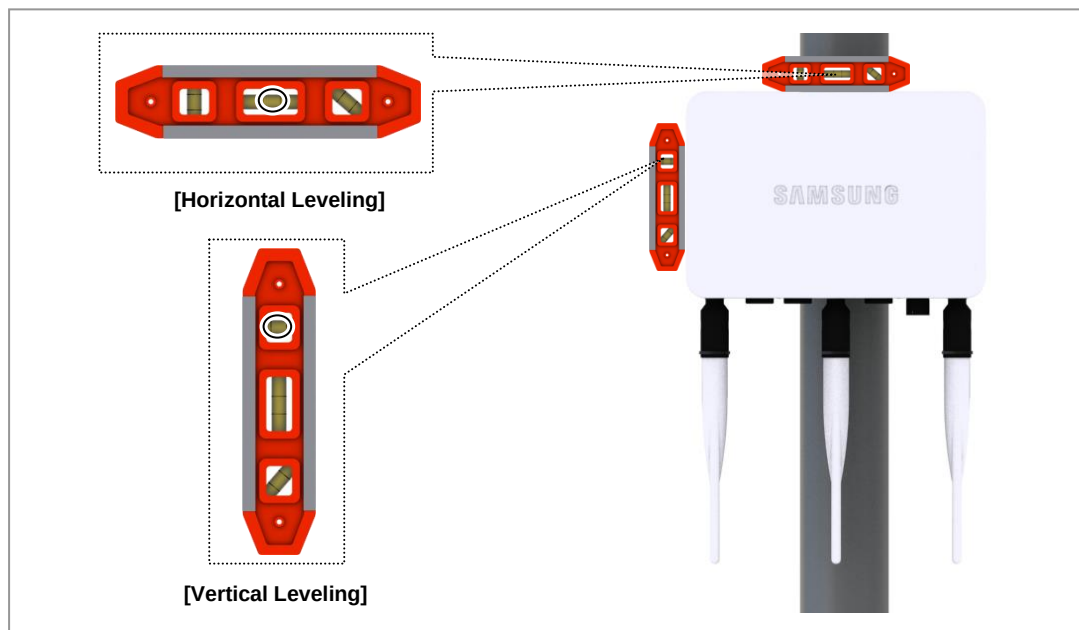
Figure 29. Using a Spirit Level on a Pole Mount (1)
