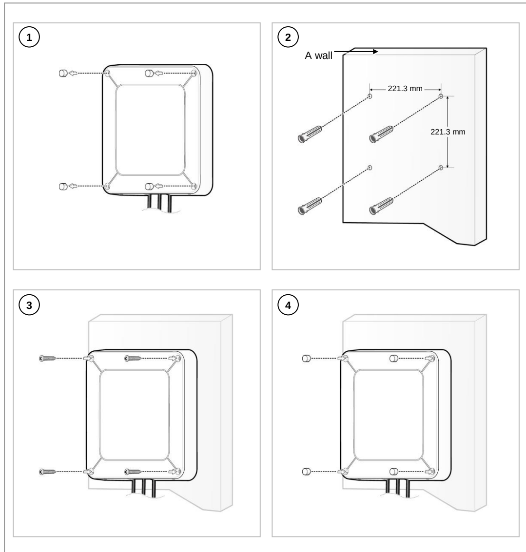
Figure 61. Installing on a Wall
