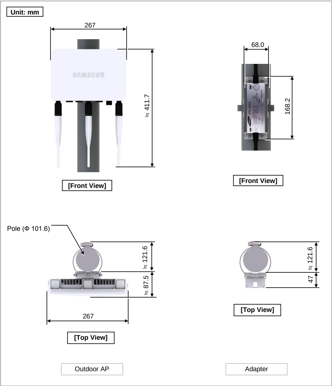
Figure 5. Pole Type Arrangement
