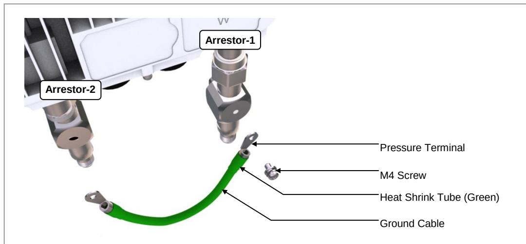
Figure 37. Connecting a Ground Cable to the Arrestor (1)
