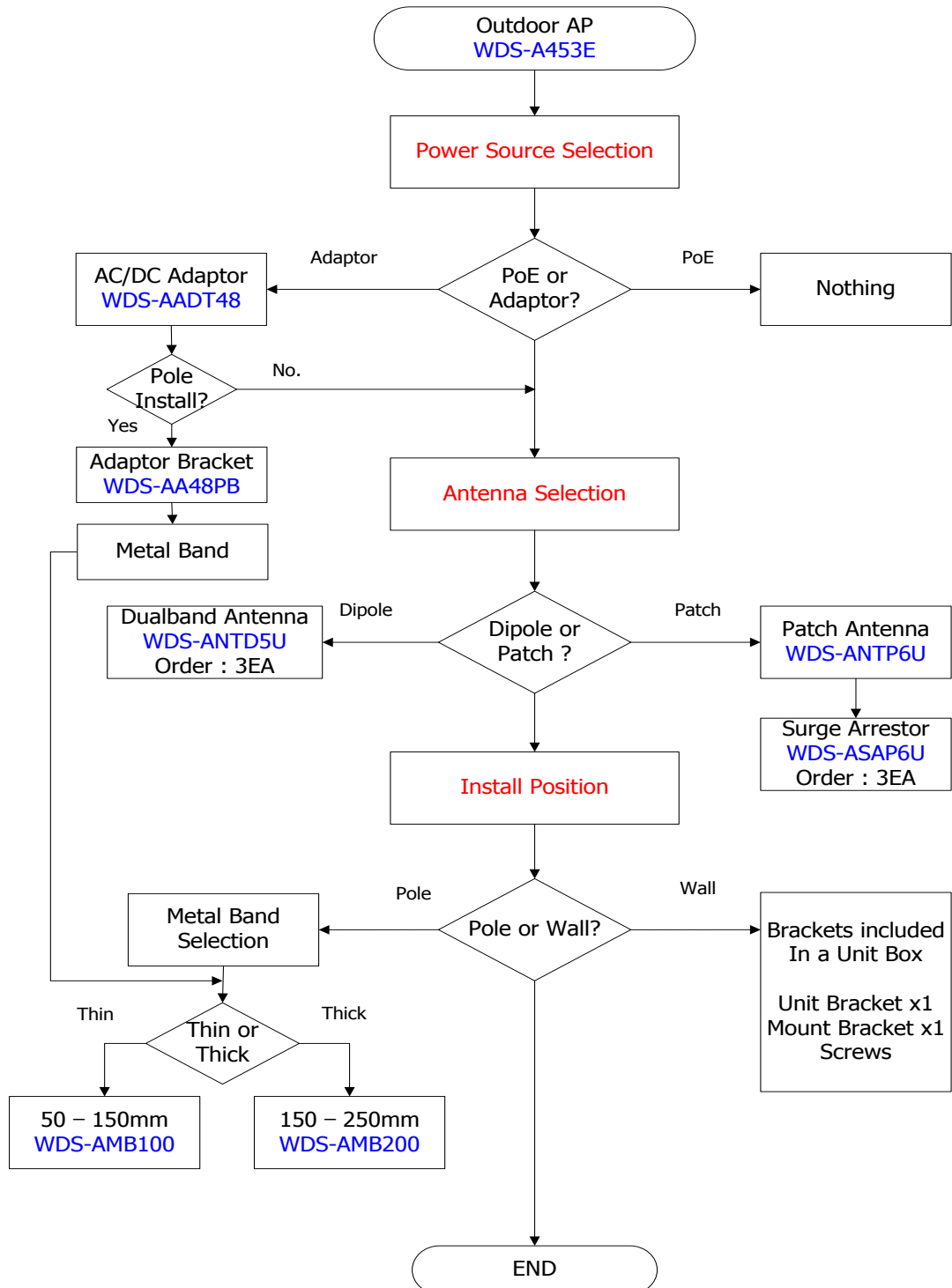
Figure 90. Outdoor AP Selection Guide
