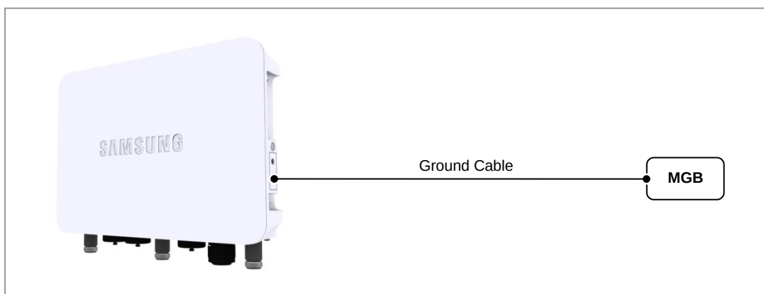
Figure 34. Connecting a Ground Cable to the Outdoor AP (1)
