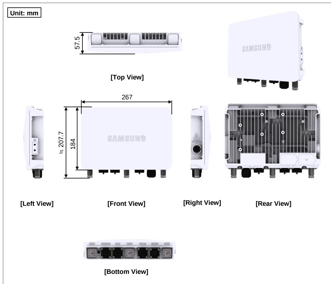
Figure 1. Outdoor AP Design
