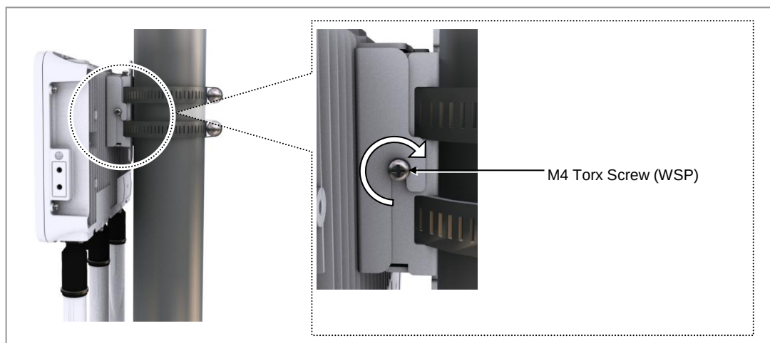
Figure 23. Mounting the Outdoor AP on a Pole (3)
