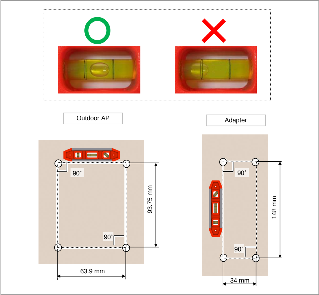
Figure 12. Marking Example
