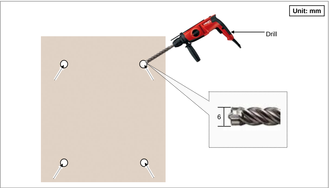
Figure 13. Drilling Example
