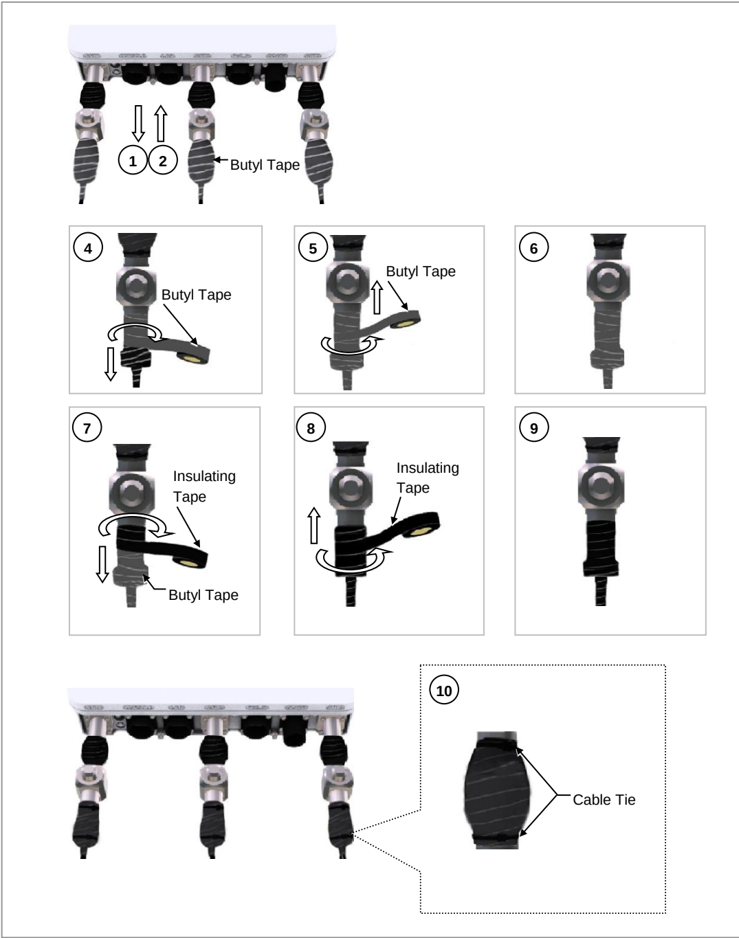
Figure 59. Connecting the Patch Antenna Cables (4)
