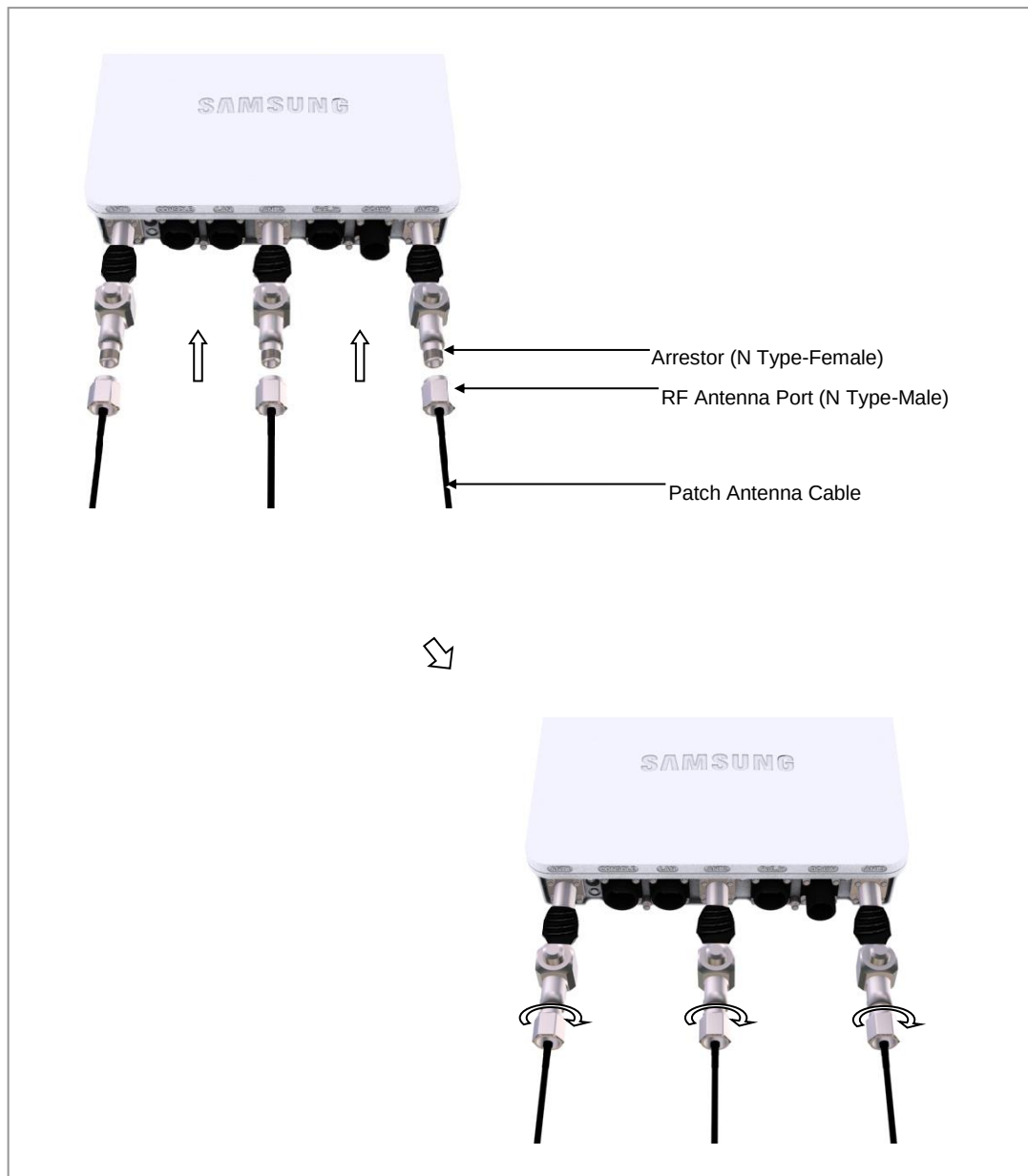
Figure 57. Connecting the Patch Antenna Cables (2)
