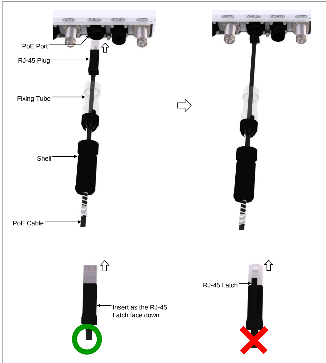
Figure 46. Connecting the PoE Cable (2)
