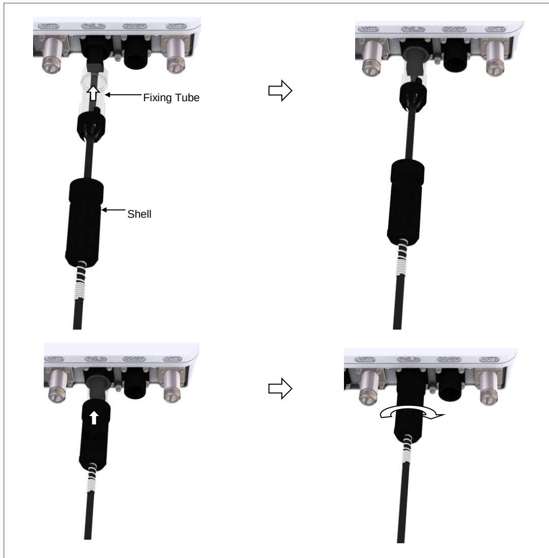
Figure 47. Connecting the PoE Cable (3)
