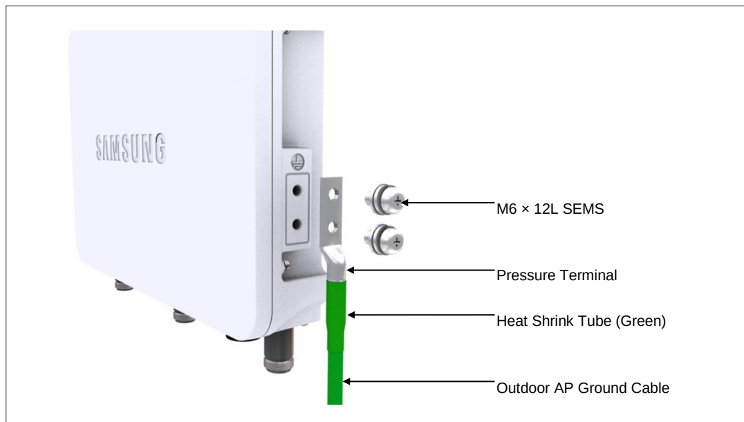
Figure 35. Connecting a Ground Cable to the Outdoor AP (2)
