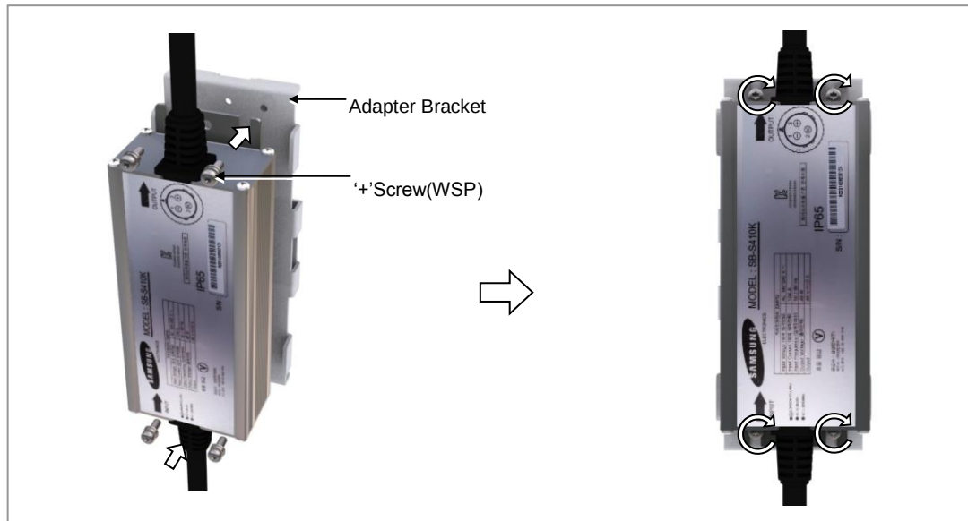
Figure 25. Mounting the Adapter on a Pole (1)
