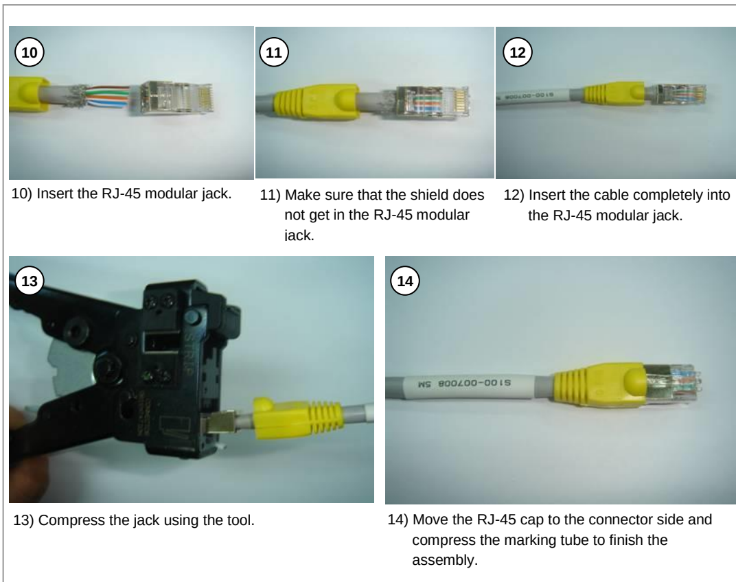
Figure 67. Assembling the RJ-45 Connector (Shield Type) (2)
