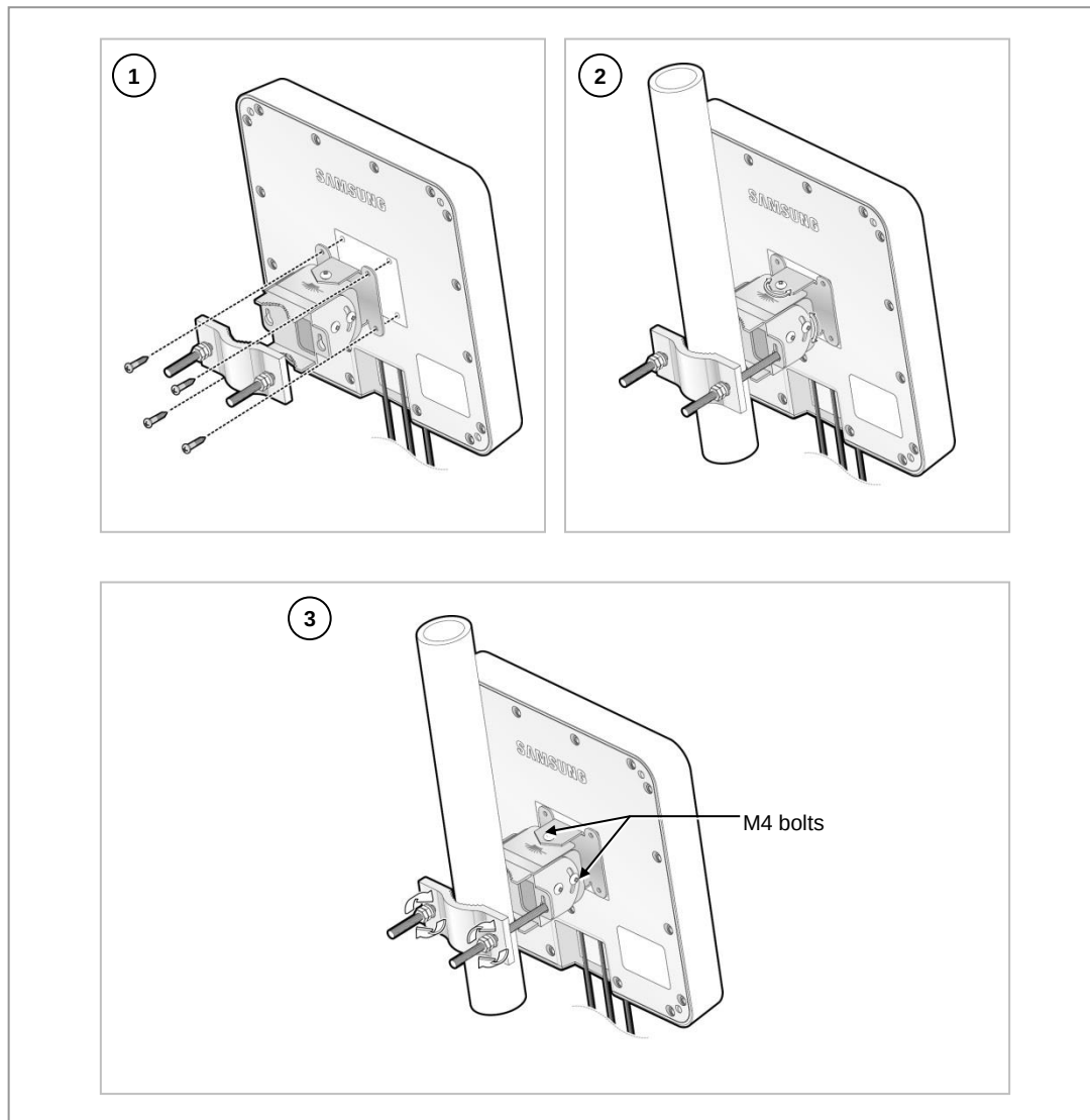
Figure 62. Installing on a Pipe
