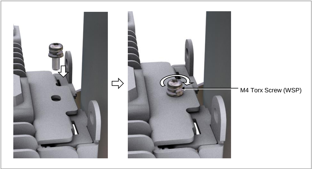
Figure 24. Mounting the Outdoor AP on a Pole (4)
