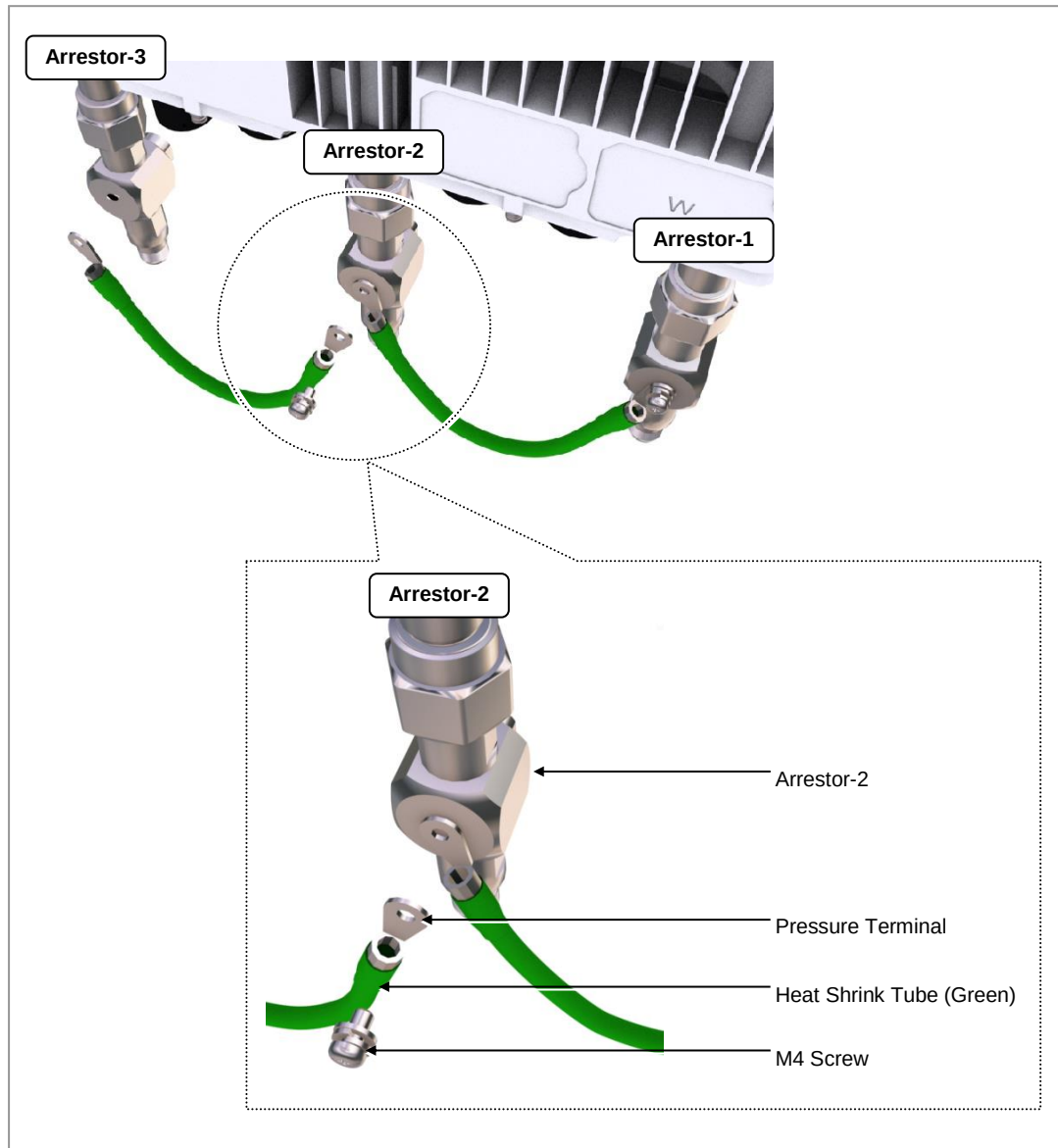
Figure 38. Connecting a Ground Cable to the Arrestor (2)
