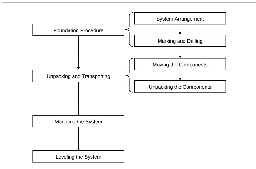
Figure 3. Installation Procedure for the Outdoor AP
