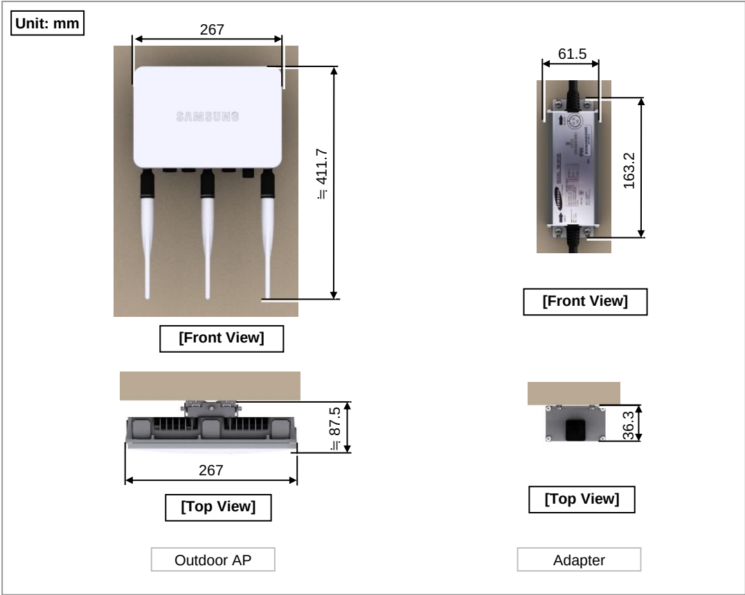
Figure 4. Wall Type Arrangement
