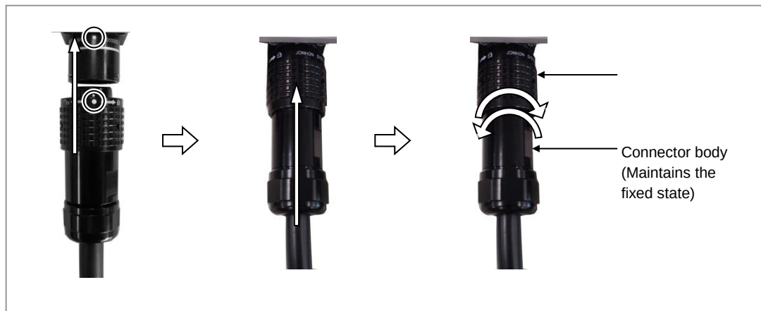
Figure 44. Connecting a Power Cable (3)
