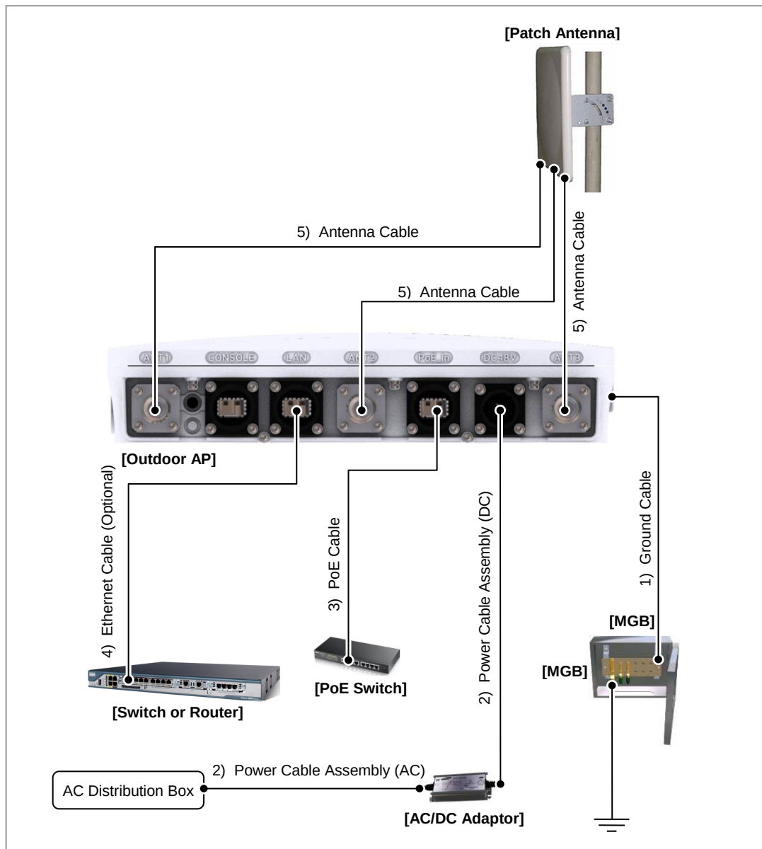
Figure 33. Outdoor AP Connection Cables
