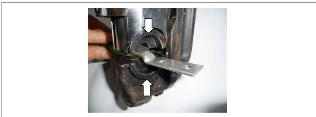
Figure 85. Fixing Pressure Terminal_Hydraulic Press (3)
