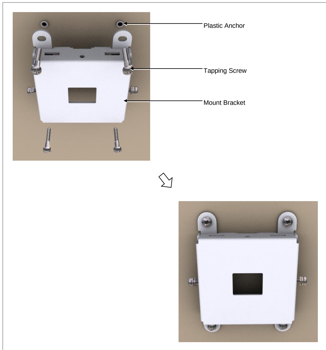
Figure 15. Mounting the Mount Bracket on the Wall (2)
