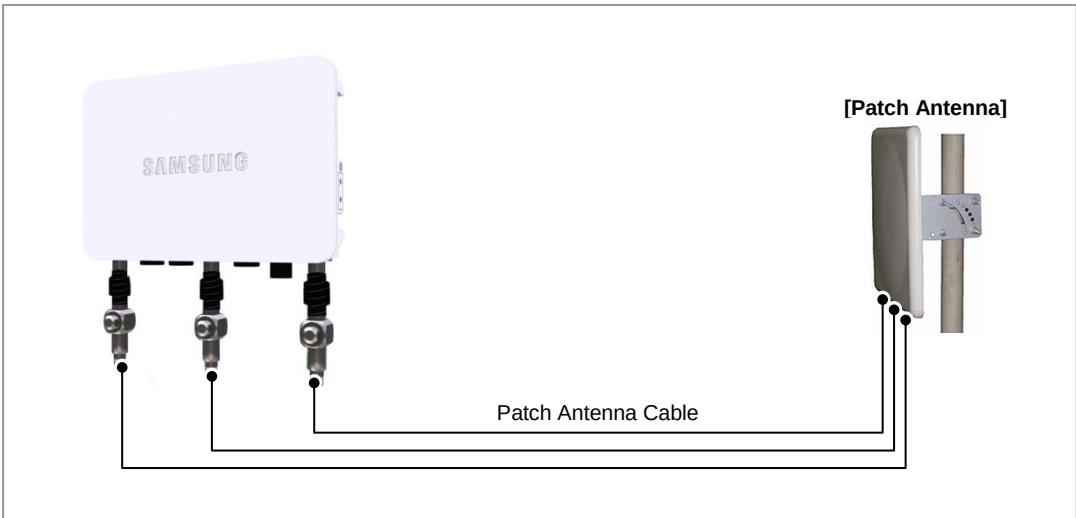
Figure 56. Connecting the Patch Antenna Cables (1)
