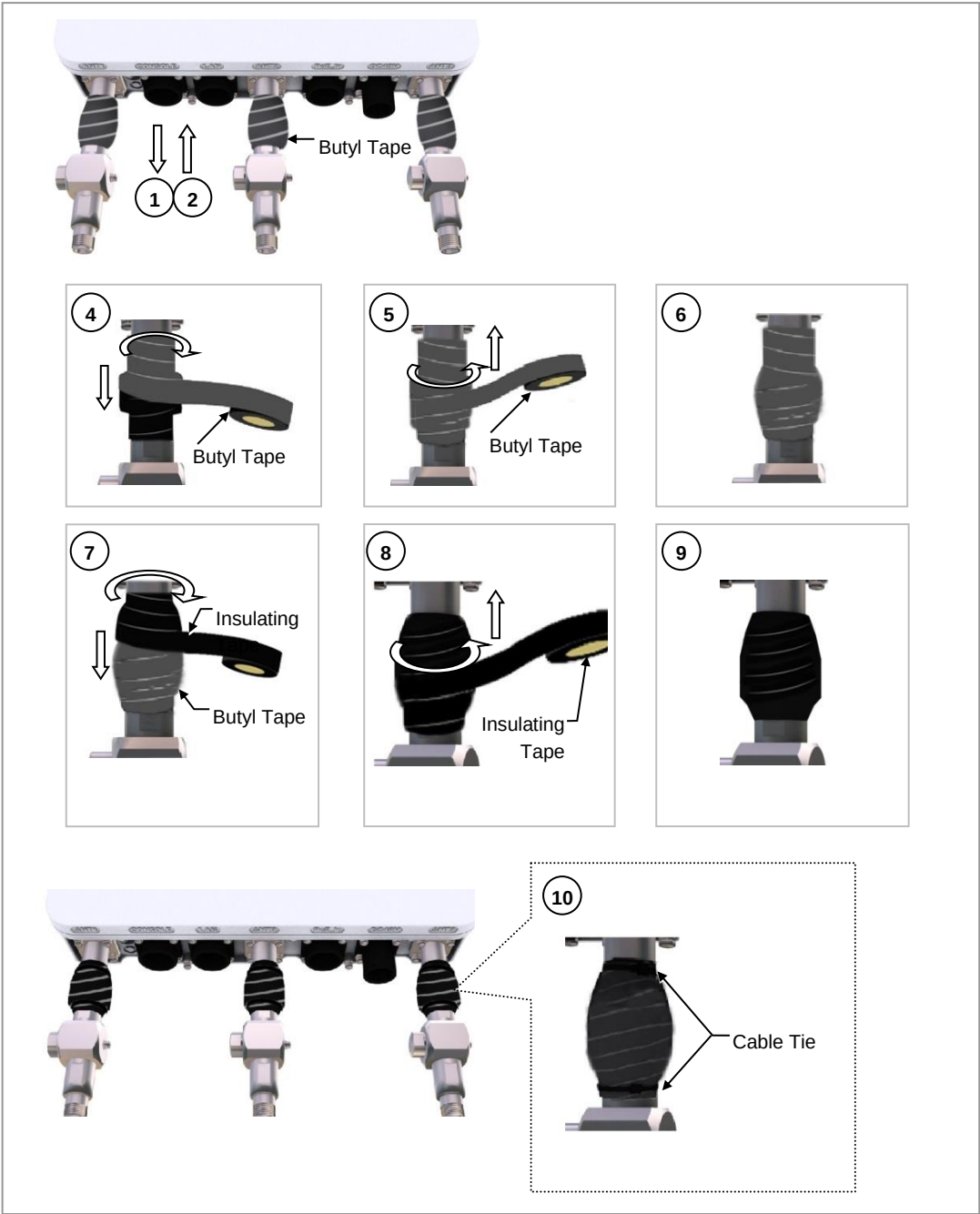
Figure 55. Connecting the Arrestors (3)
