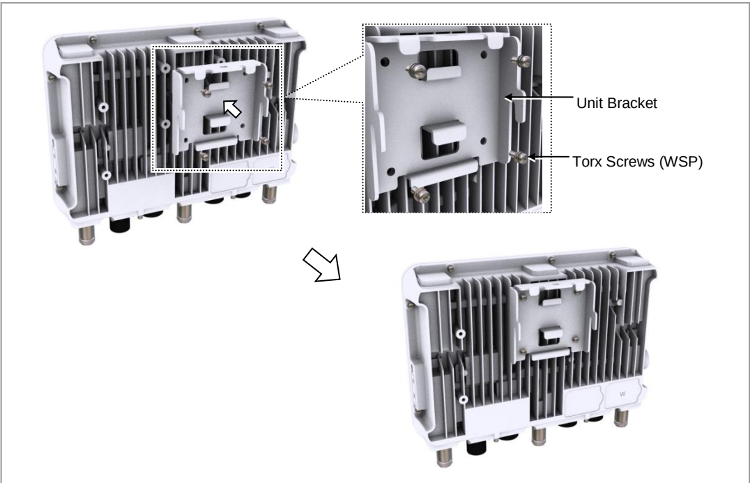
Figure 6. Assembling the Unit Bracket
