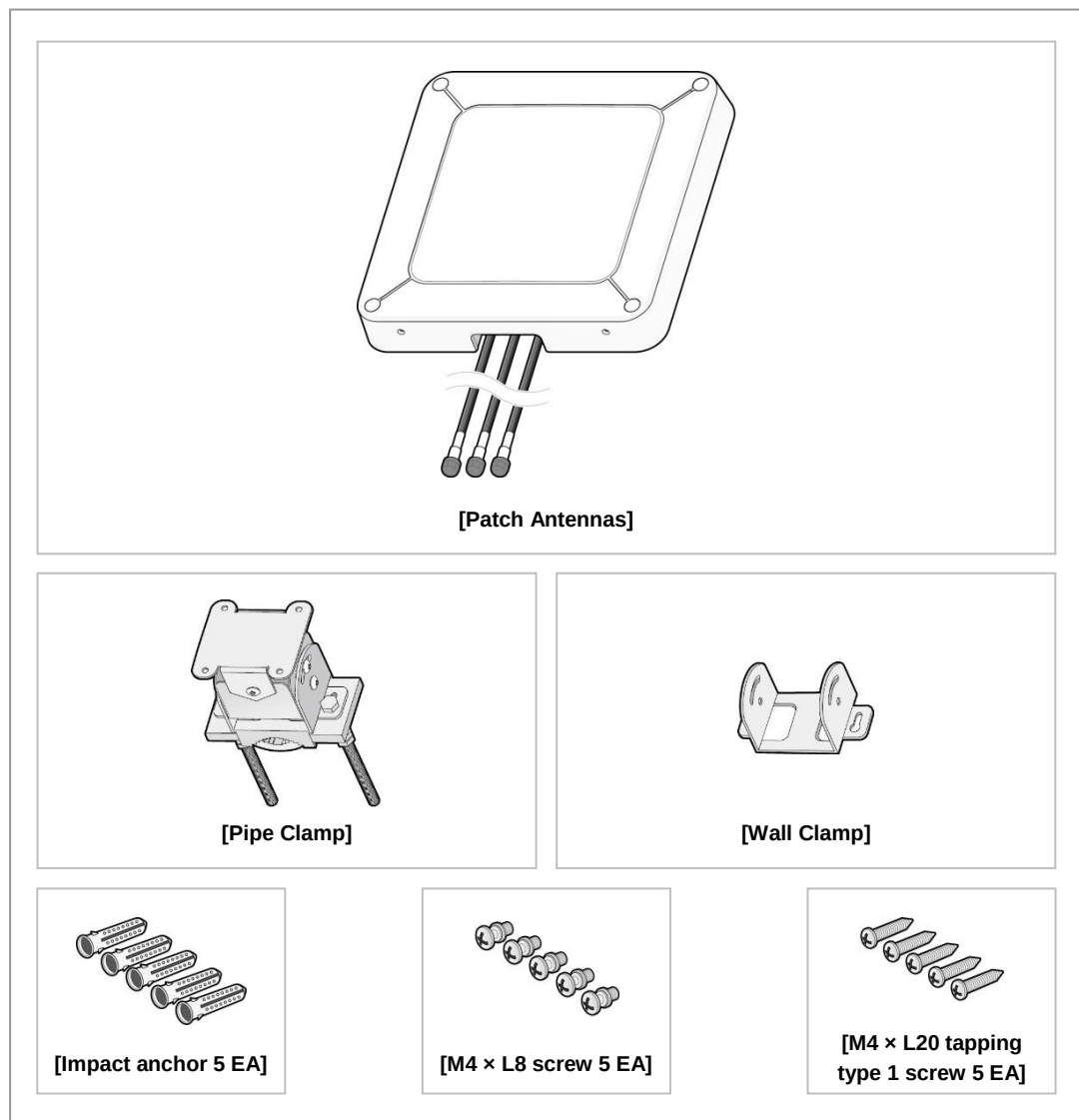
Figure 60. Patch Antenna Package Components
