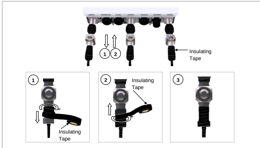
Figure 58. Connecting the Patch Antenna Cables (3)
