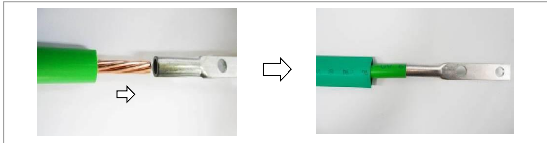
Figure 78. Fixing Pressure Terminal_Handheld Compressor (1)
