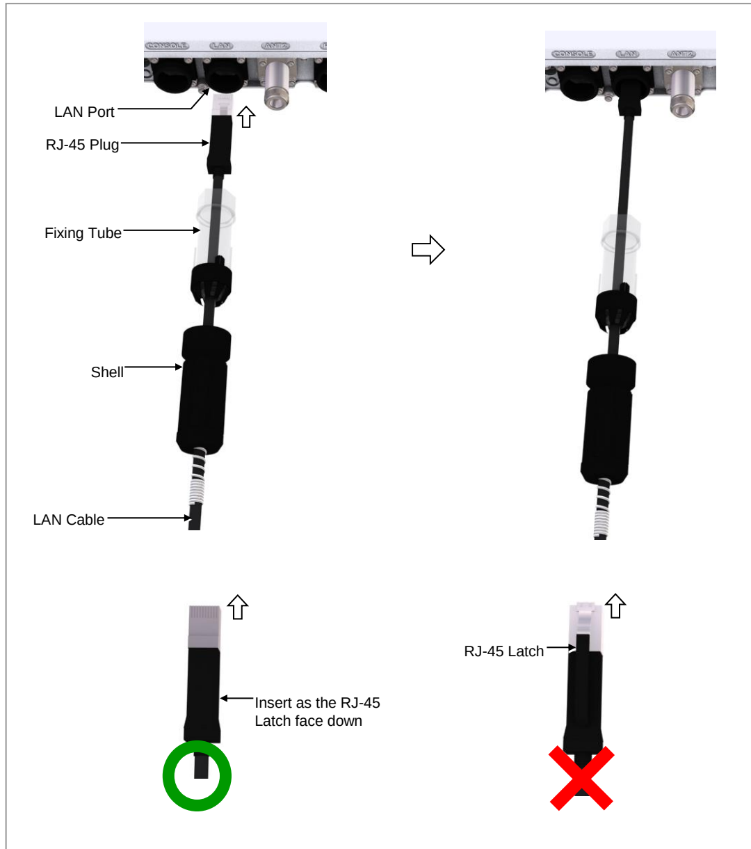
Figure 50. Connecting a LAN Cable (2)
