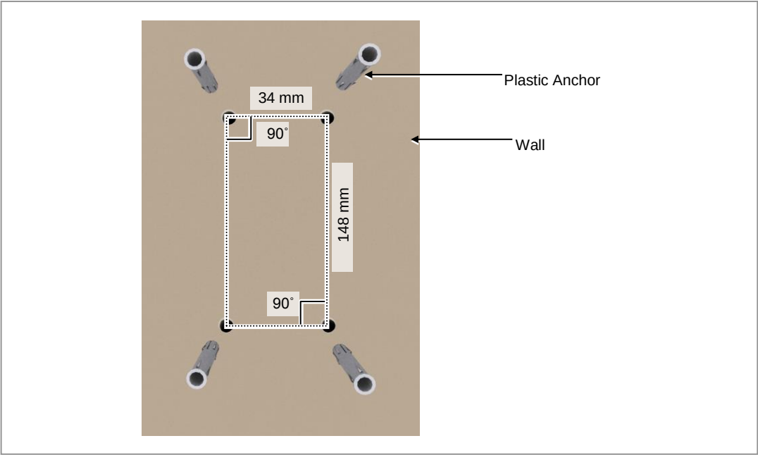
Figure 19. Mounting the Adapter (1)
