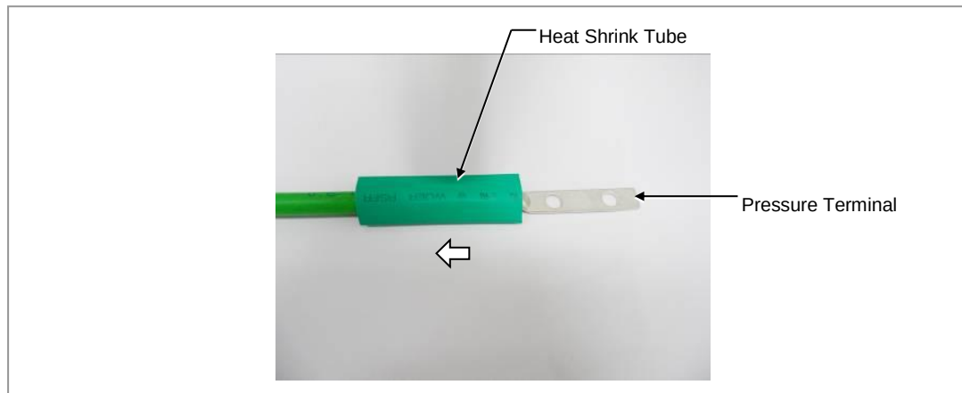
Figure 88. Assembling Heat Shrink Tube (1)
