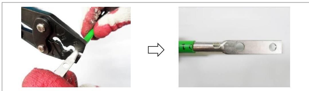
Figure 80. Fixing Pressure Terminal_Handheld Compressor (3)
