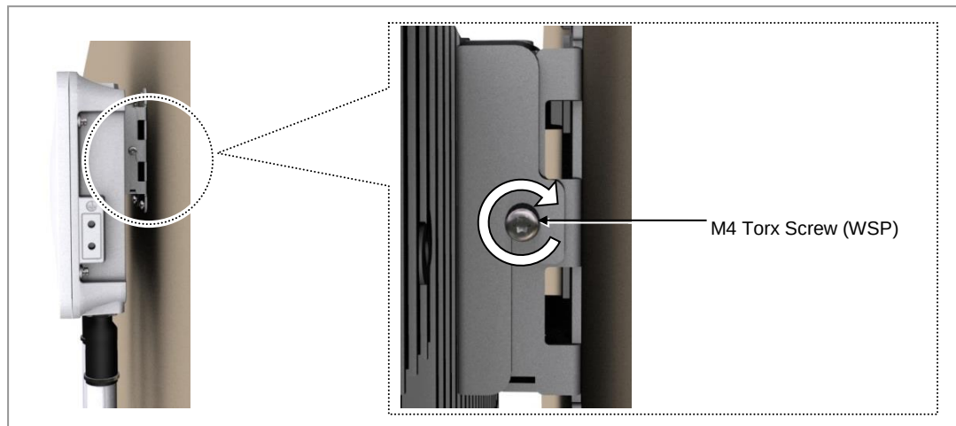
Figure 17. Mounting the Outdoor AP on the Wall (2)
