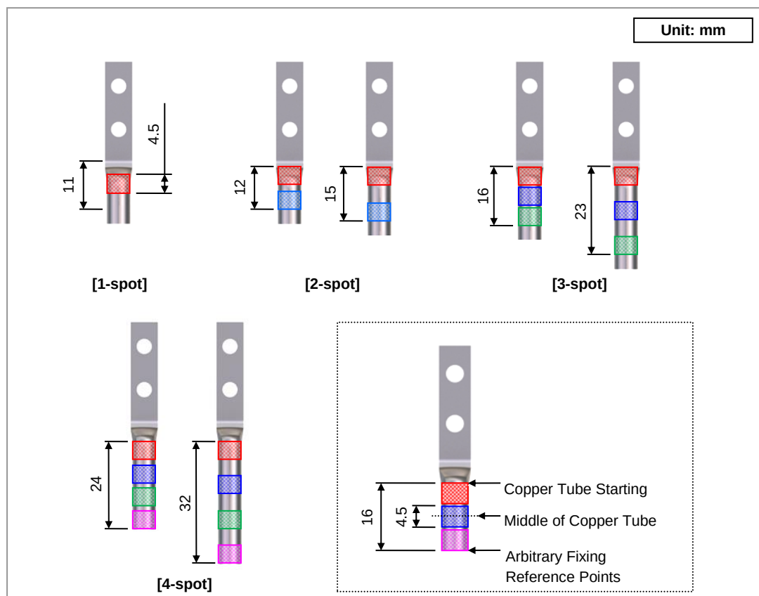
Figure 70. Pressure Reference Drawing (Handheld Compressor)
