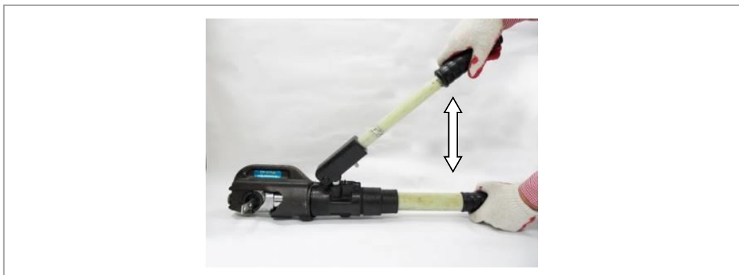
Figure 86. Fixing Pressure Terminal_Hydraulic Press (4)
