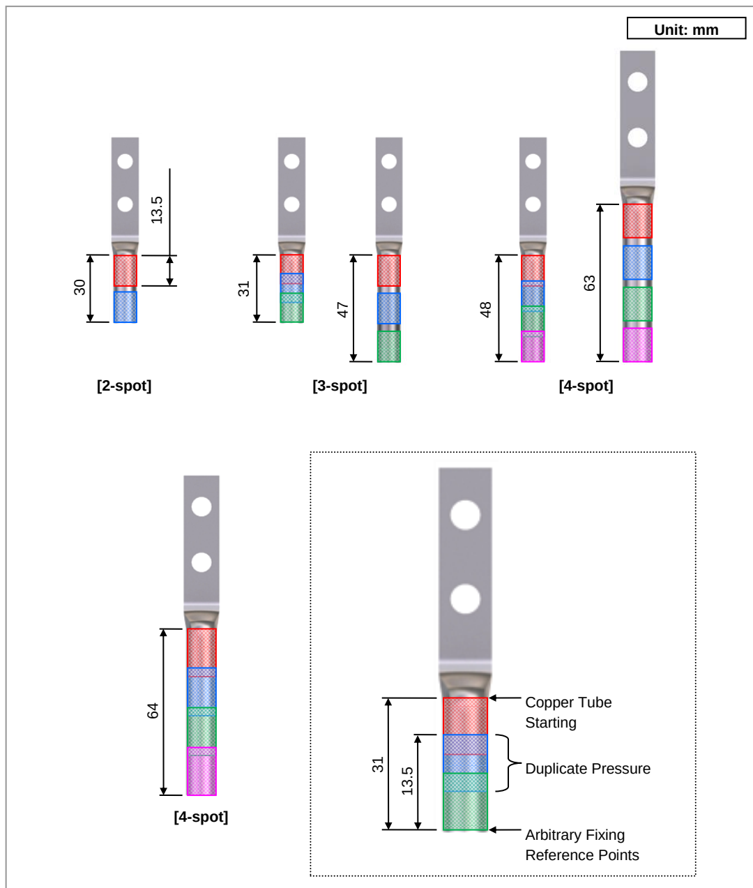
Figure 71. Pressure Reference Drawing (Hydraulic Compressor)
