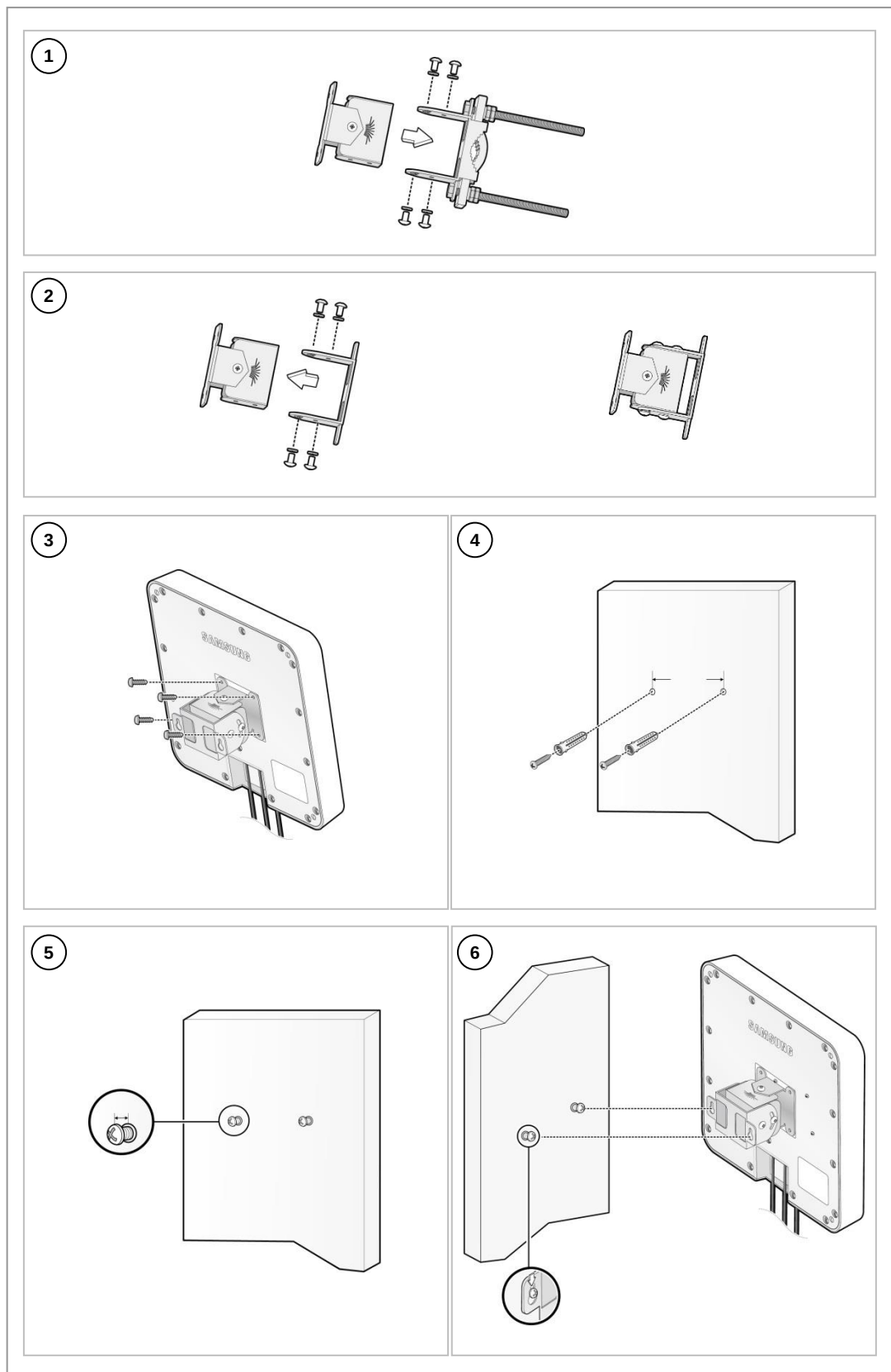
Figure 63. Installing on a Wall Using Brackets
