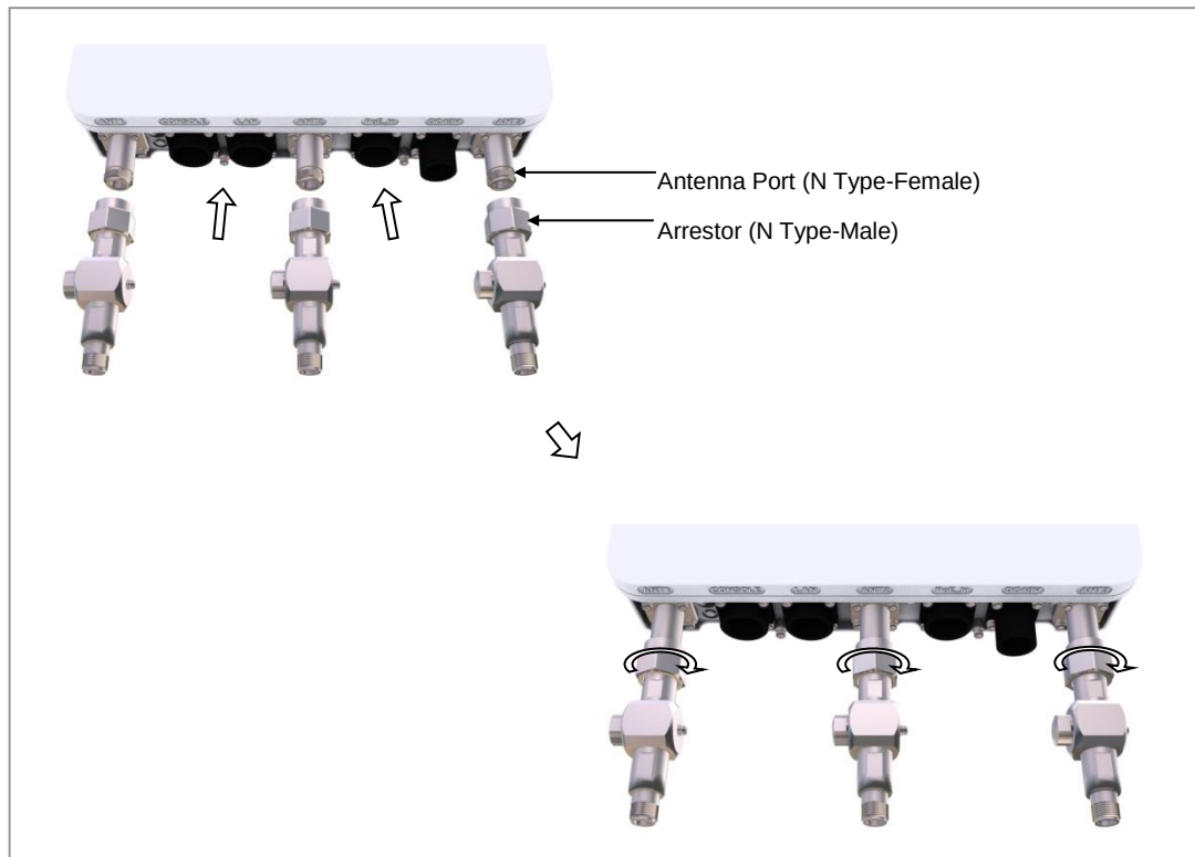
Figure 53. Connecting the Arrestors (1)
