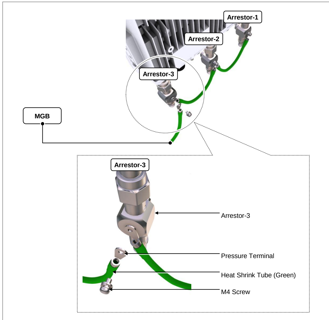
Figure 39. Connecting a Ground Cable to the Arrestor (3)
