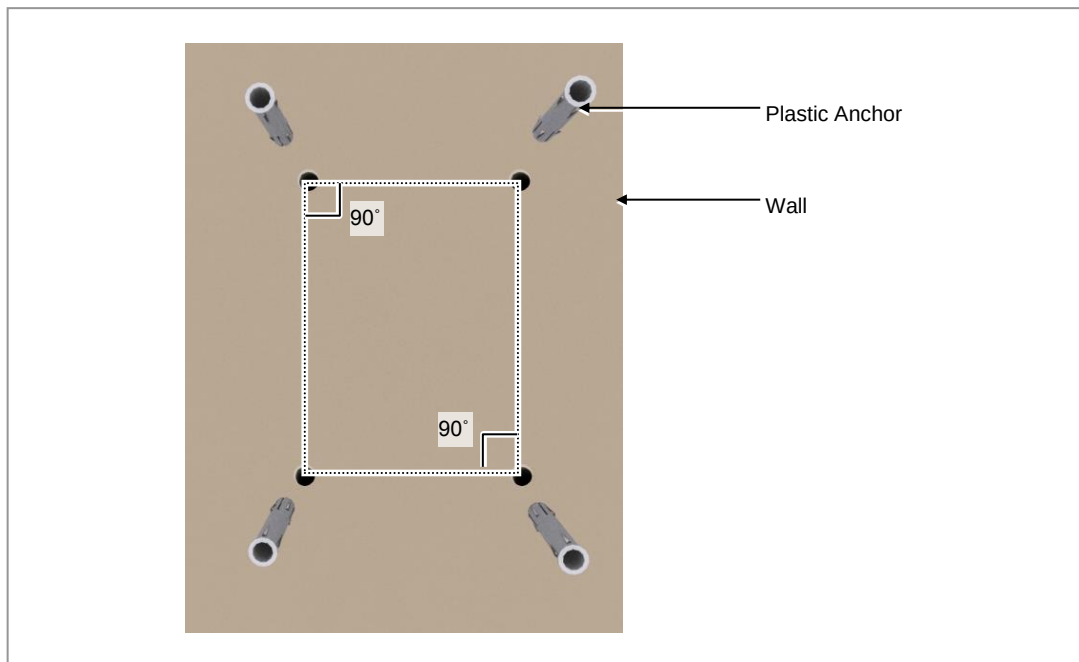
Figure 14. Mounting the Mount Bracket on the Wall (1)
