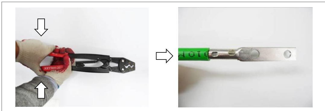
Figure 82. Fixing Pressure Terminal_Handheld Compressor (5)
