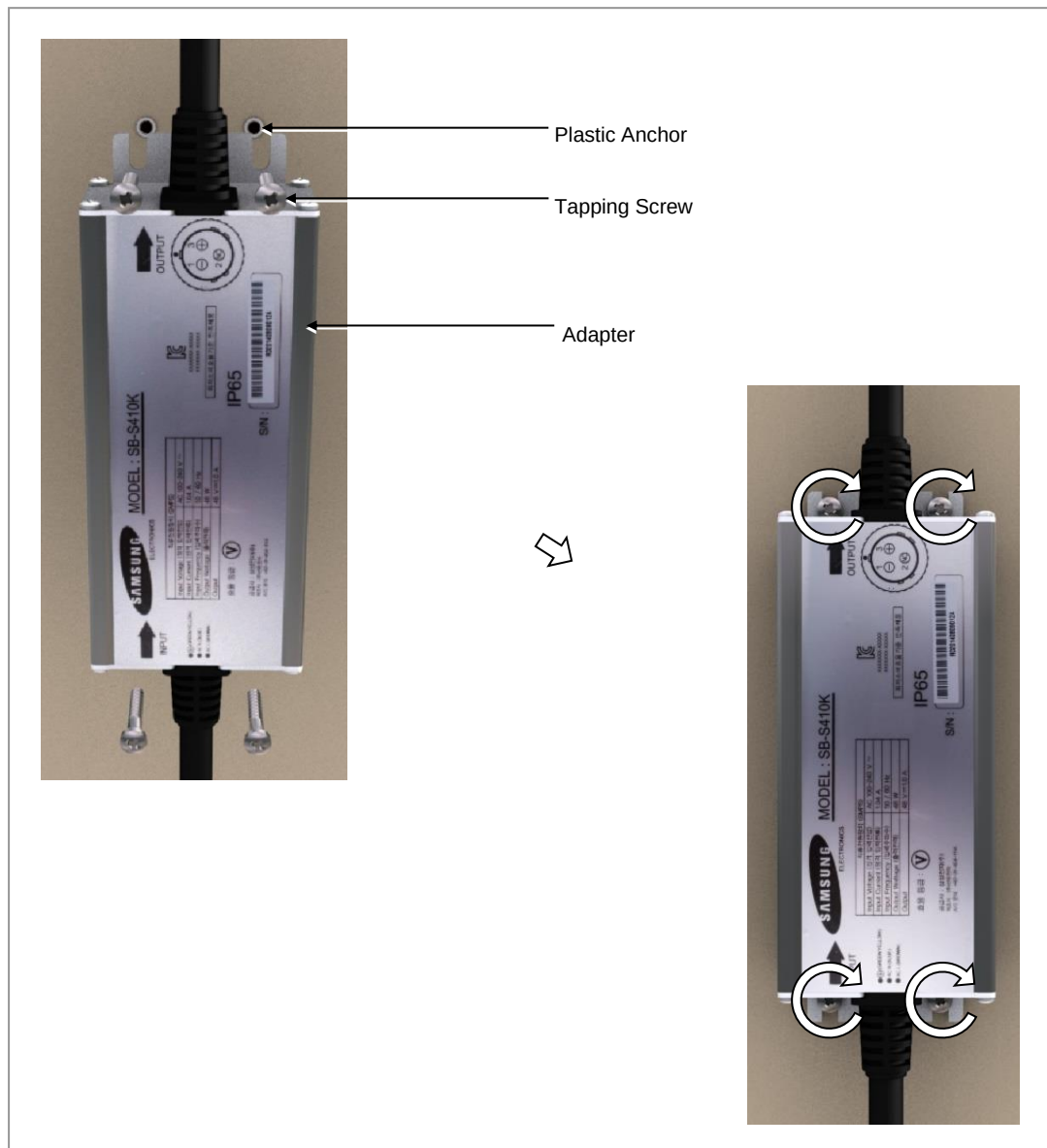
Figure 20. Mounting the Adapter (2)
