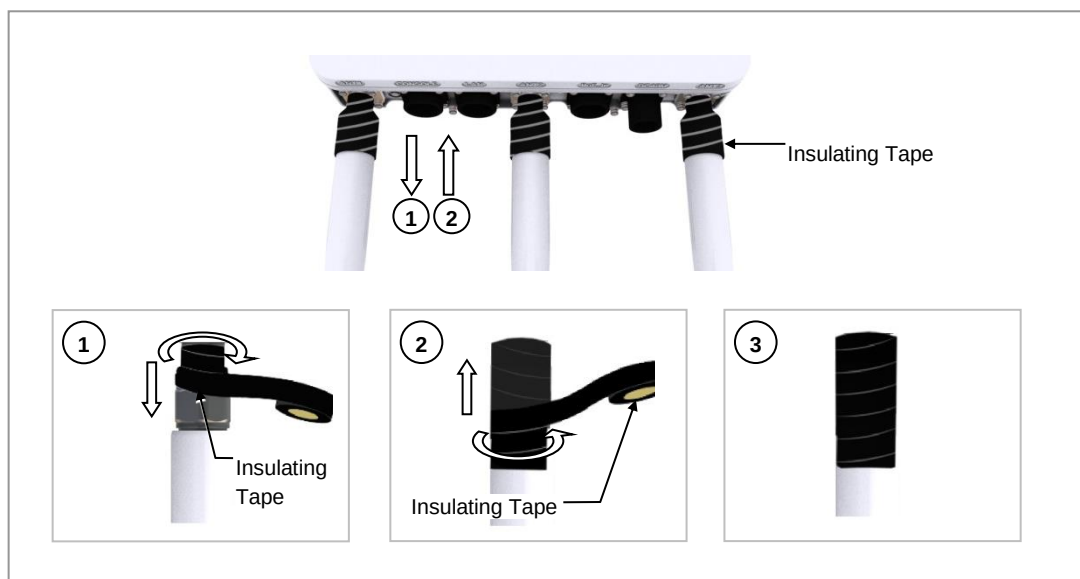
Figure 8. Assembling the Dipole Antennas (2)
