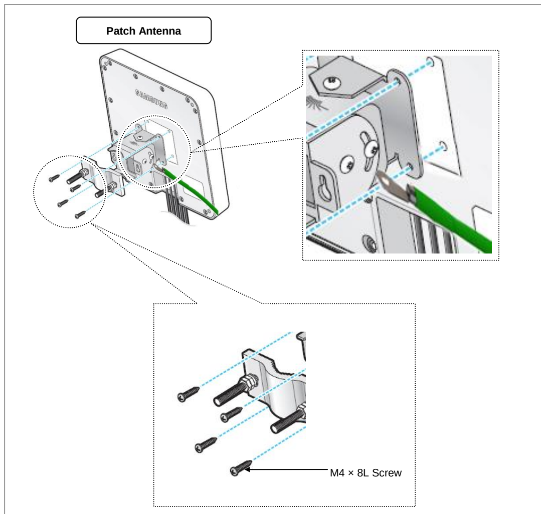
Figure 40. Connecting a Ground Cable to the Patch Antenna
