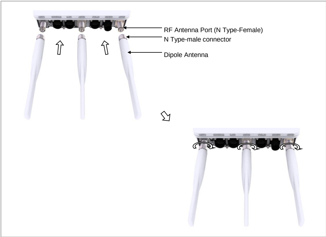
Figure 7. Assembling the Dipole Antennas (1)
