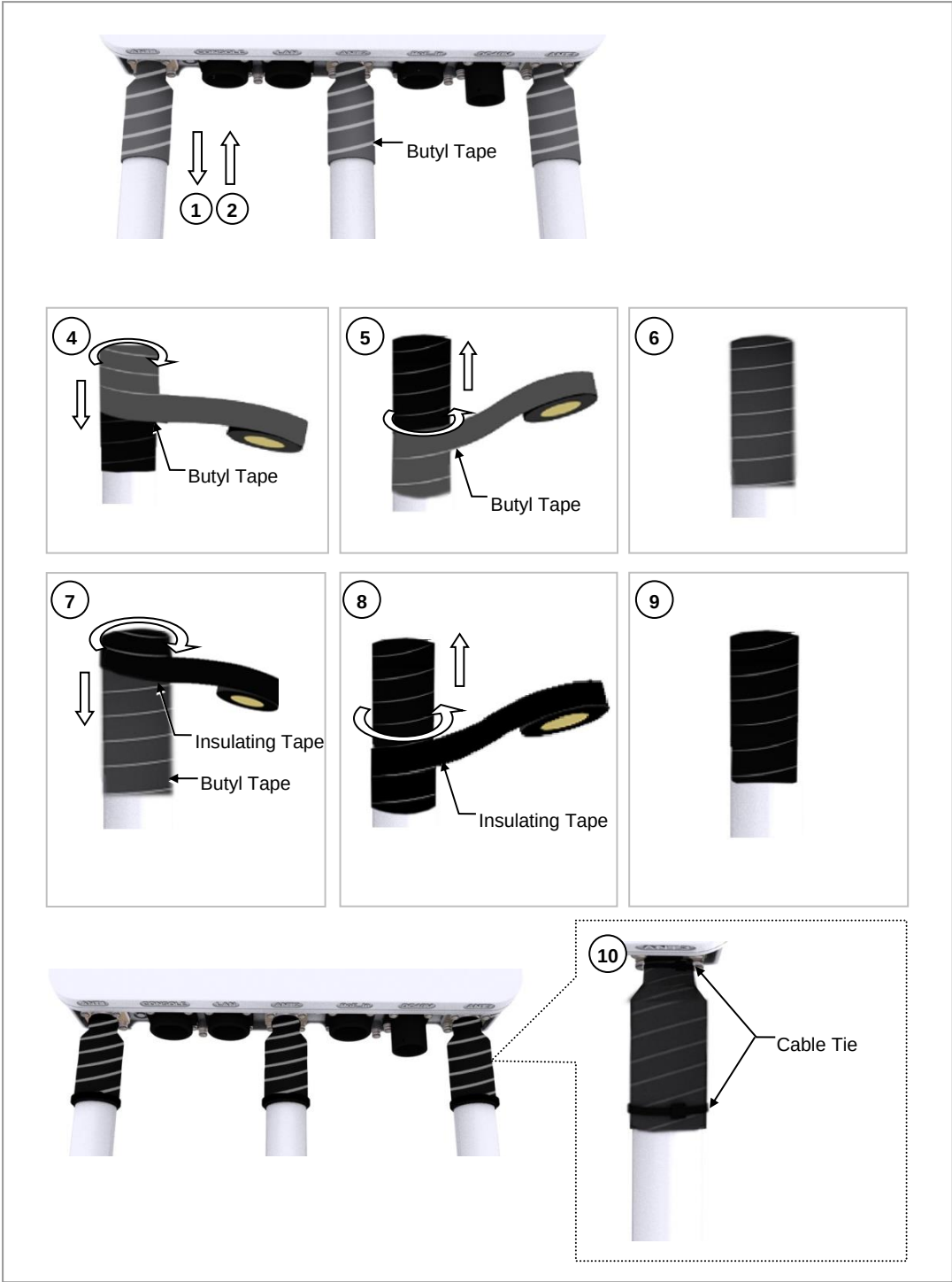
Figure 9. Assembling the Dipole Antennas (3)
