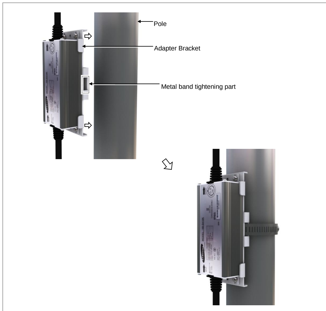
Figure 26. Mounting the Adapter on a Pole (2)
