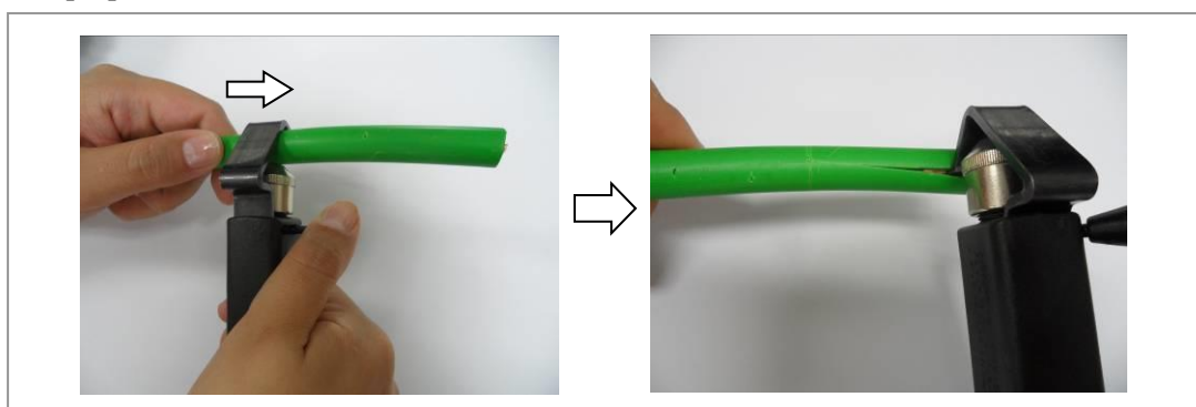
Figure 76. Stripping Cable Sheath (5)
