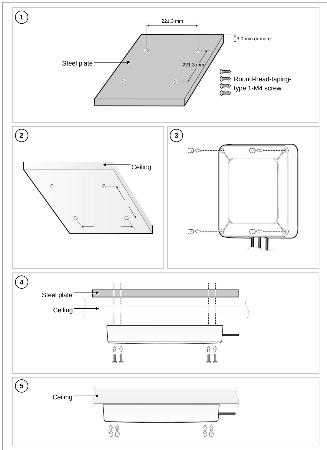
Figure 64. Installing on a Ceiling
