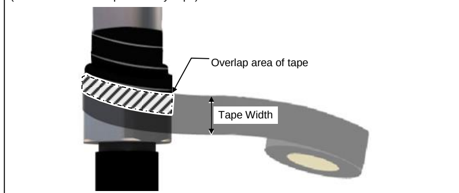
Figure 68. Check Items for Finishing the Connector Connection Part
