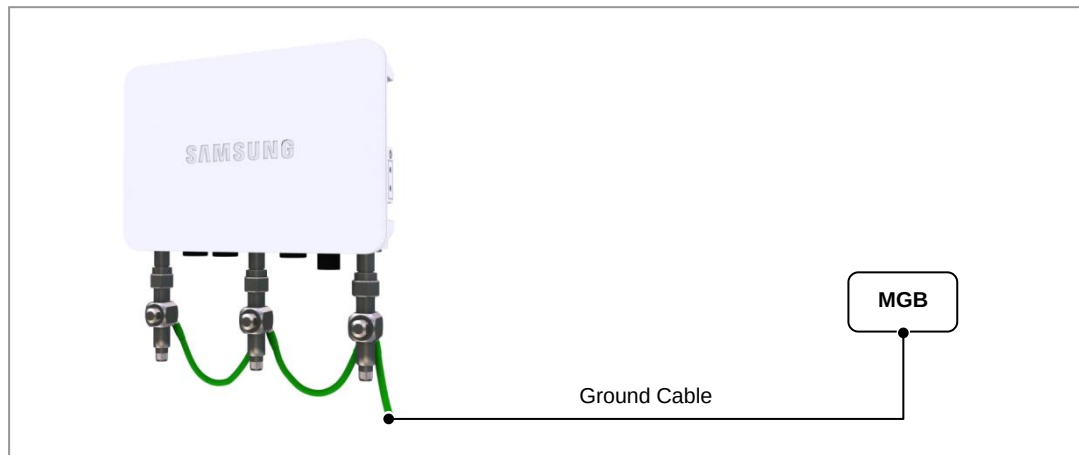
Figure 36. Connecting a Ground Cable to the Outdoor AP (3)
