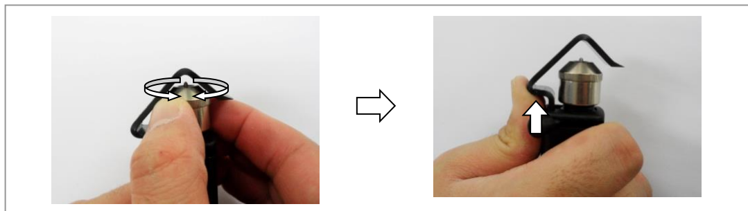
Figure 73. Stripping Cable Sheath (2)
