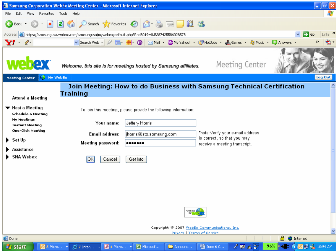
Figure 4 – Login Window
