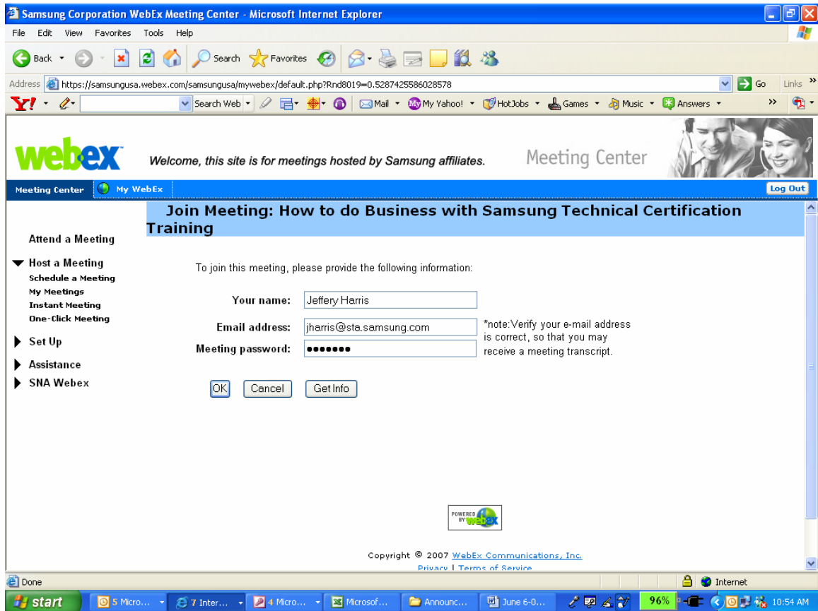
Figure 4 – Login Window
