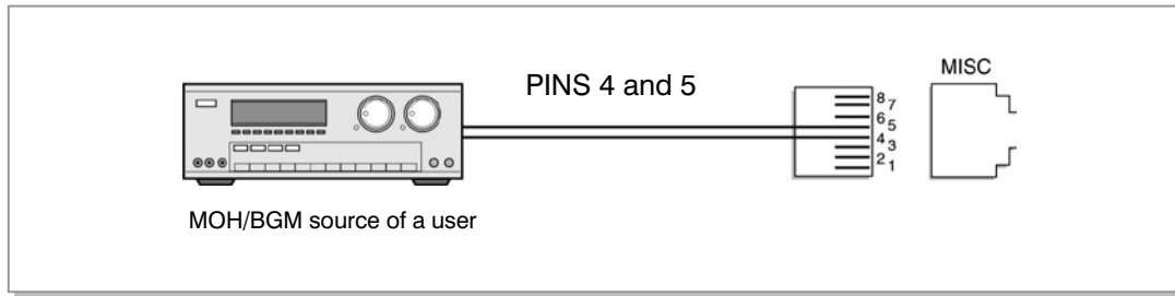
Figure 7.24 Connecting MOH/BGM Sources
