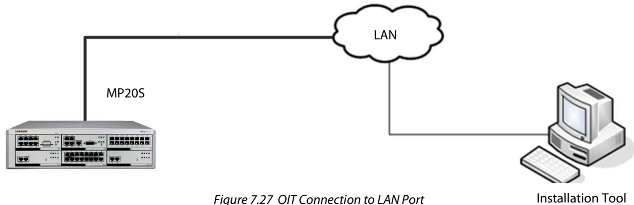
Figure 7.27 OIT Connection to LAN Port
