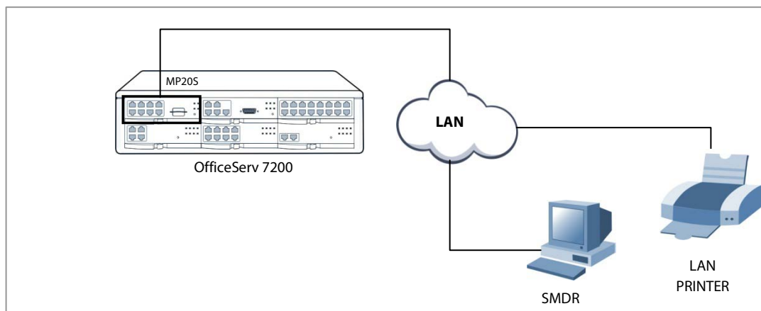
Figure 7.30 Connecting SMDR and Printer
