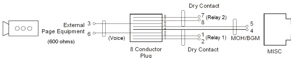
Figure 7.25 Connecting External/Additional Page Equipment
