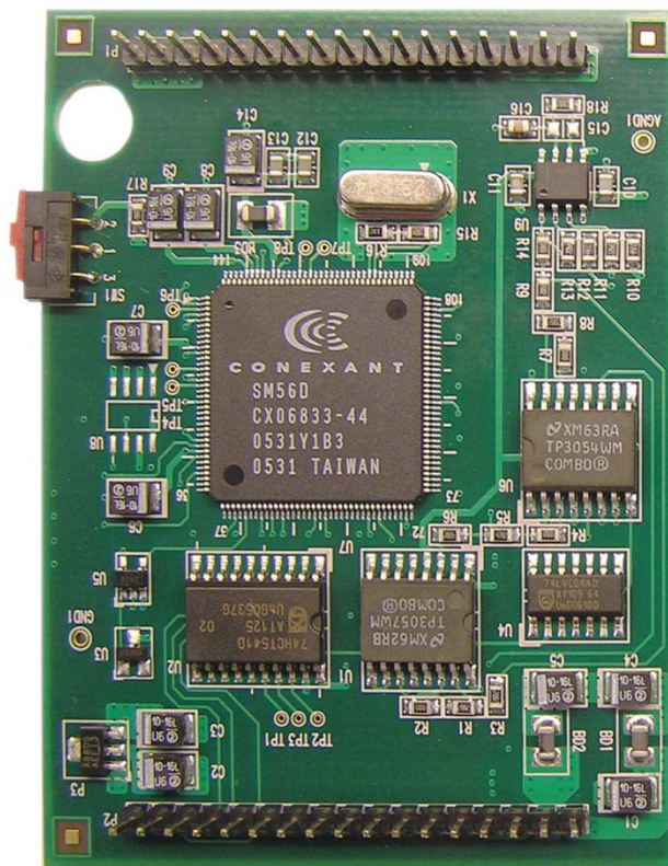
Figure 3.39 Modem Card
