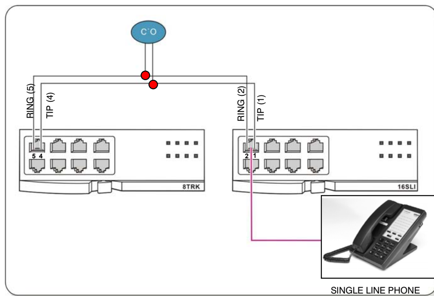
Figure 3.43 Power Fail Transfer Connection to 16MWSLI/16SLI2/8SLI/8SLI2
