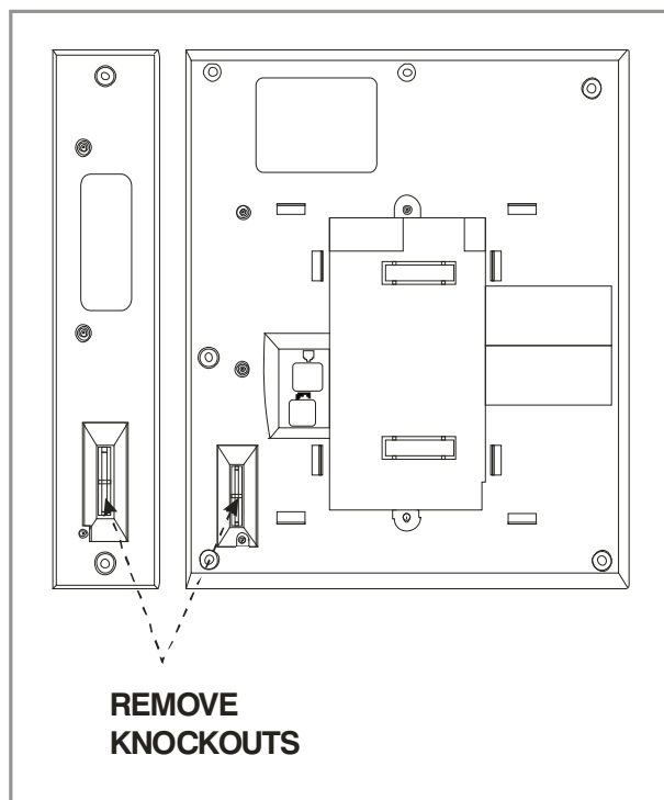
Figure 7.17 Attaching iDCS 14 Button AOM to an iDCS Keyset
