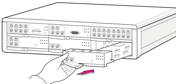
Figure 3.11 Installing Interface Board into Slot
